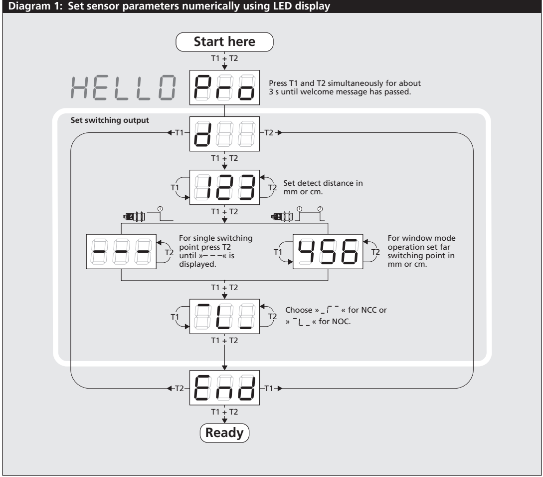
Diagram 1: Set sensor parameters numerically using LED display
