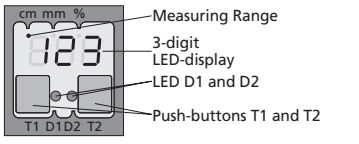
Fig. 2: TouchControl/LED display
