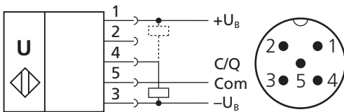
Fig. 3: Connection diagram of the pico+ sensor
